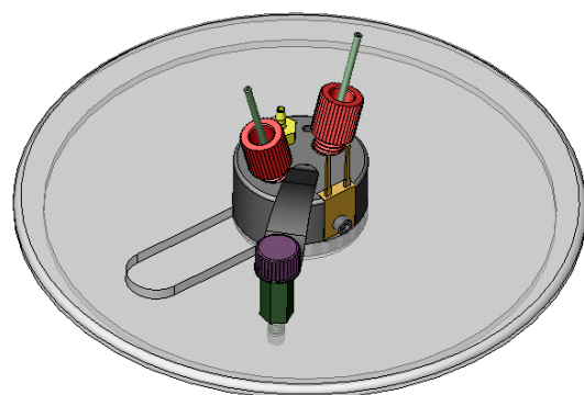
Model VC-LFR-18-H Vacu-Cell shown in a Model VC-RSH-NIK Nikon microscope stage holder
