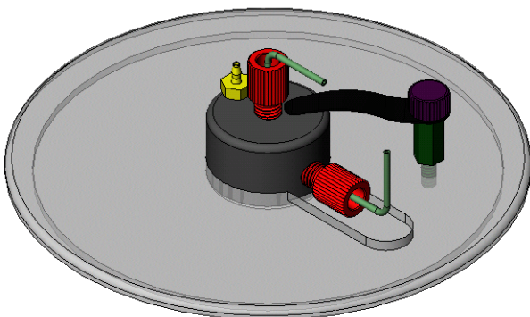
Model VC-CPR-25 Vacu-Cell shown in a Model VC-RSH-NIK Nikon microscope stage holder
